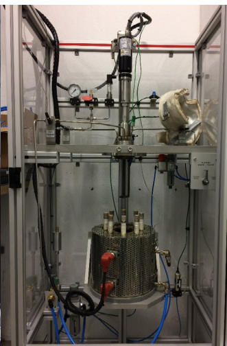
Solvolysereactor Certech
